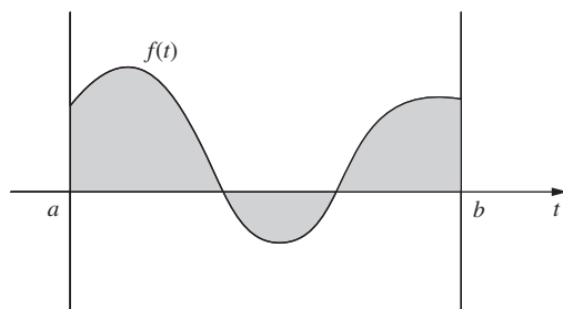
(a) \|f\|_1 is shaded
