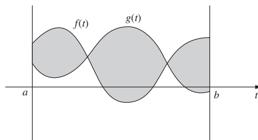
(b) d_1(f, g) is shaded
