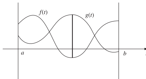
(b) d_\infty(f, g)
